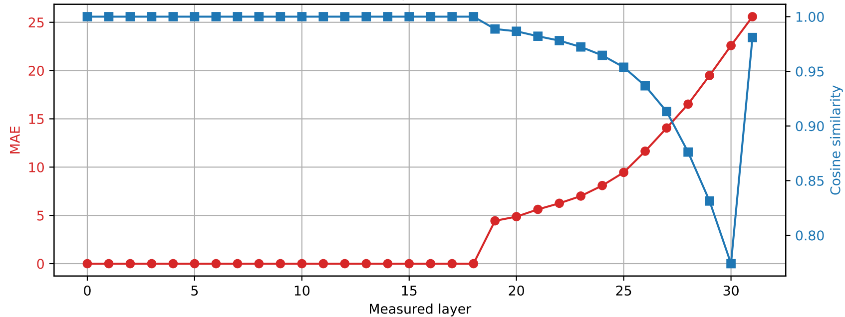
SmolLM2-360M | Prompt 4 Spared layer 18 | Hybrid vs quantized
