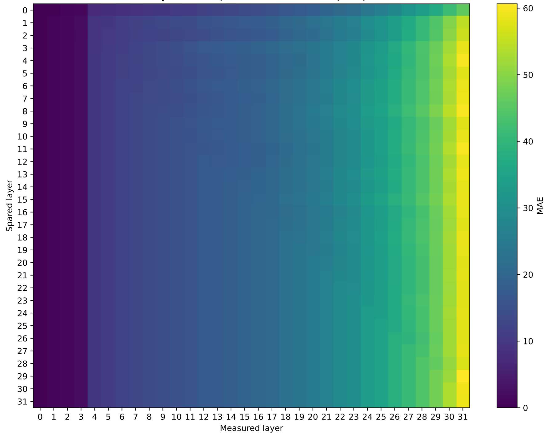
SmolLM2-360M Mean hybrid vs unquantized MAE across 5 prompts
