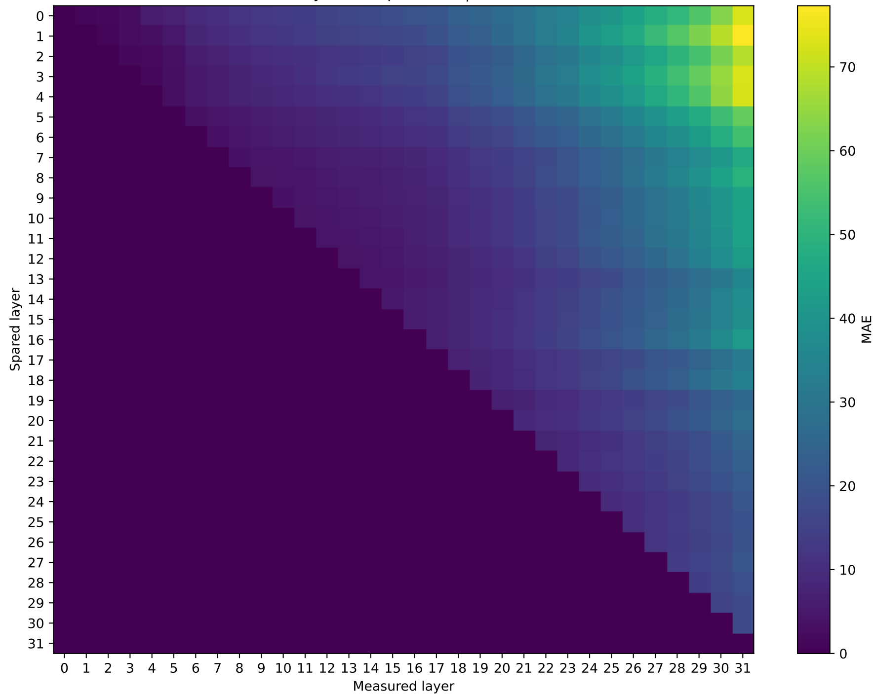
SmolLM2-360M | Prompt 0 Hybrid vs quantized | int4
