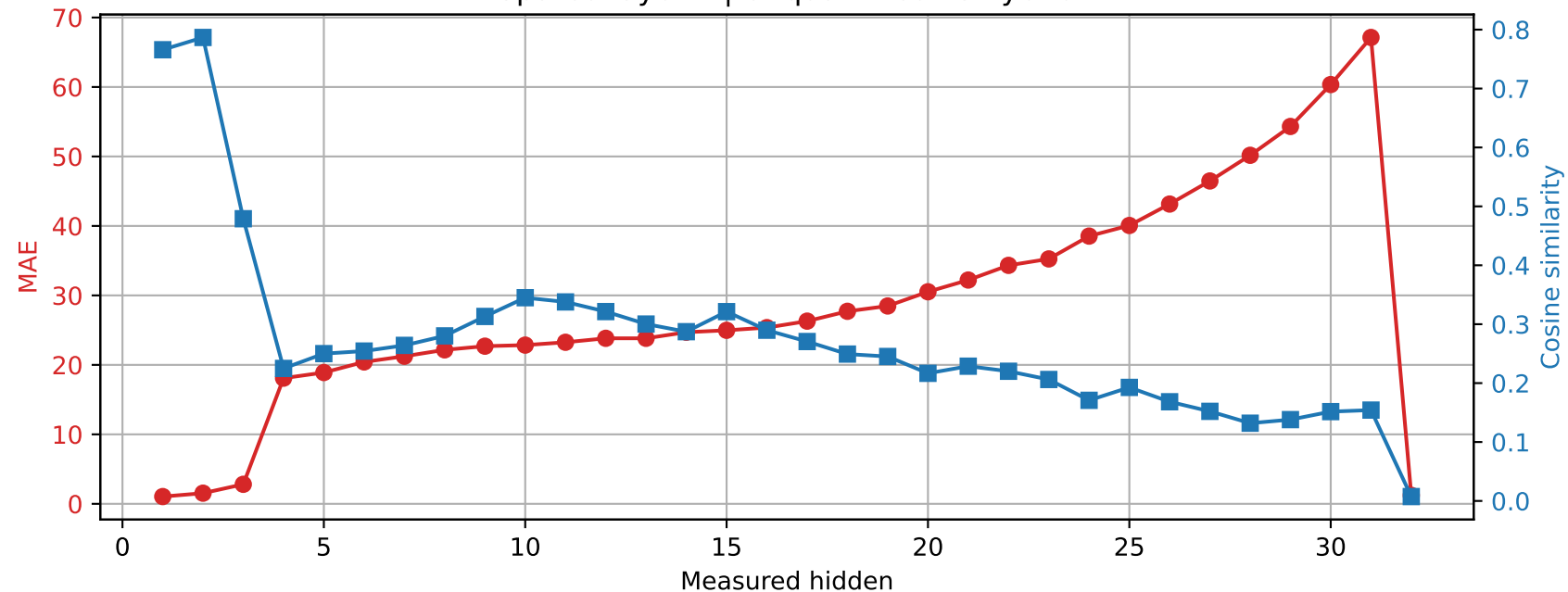
SmolLM2-360M | Prompt 0 Spared layer 1 | Unquantized vs hybrid
