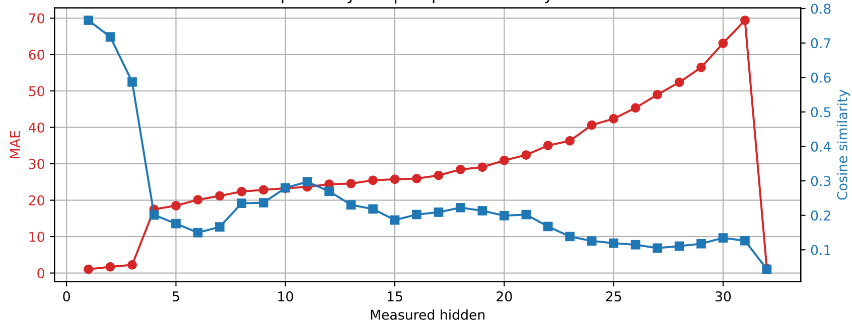
SmolLM2-360M | Prompt 0 Spared layer 2 | Unquantized vs hybrid
