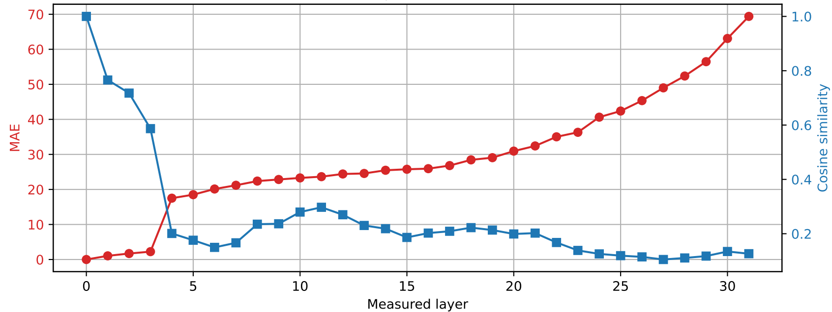
SmolLM2-360M | Prompt 0 Spared layer 2 | Hybrid vs unquantized
