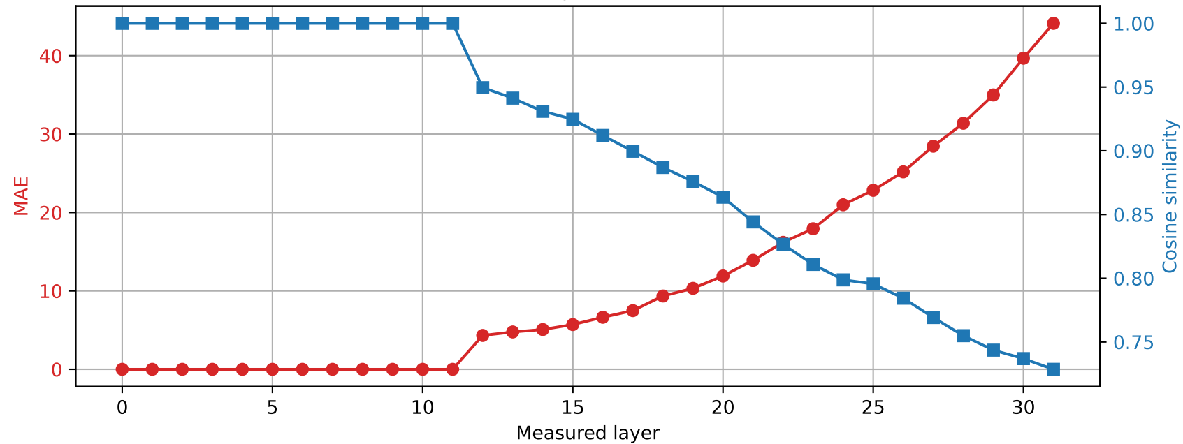
SmolLM2-360M | Prompt 0 Spared layer 11 | Hybrid vs quantized
