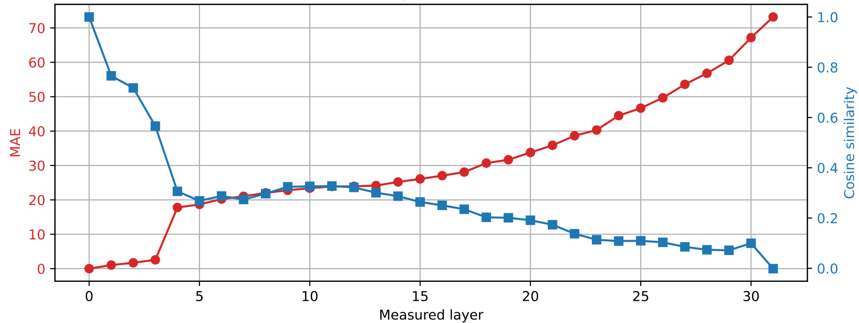
SmolLM2-360M | Prompt 0 Spared layer 11 | Hybrid vs unquantized
