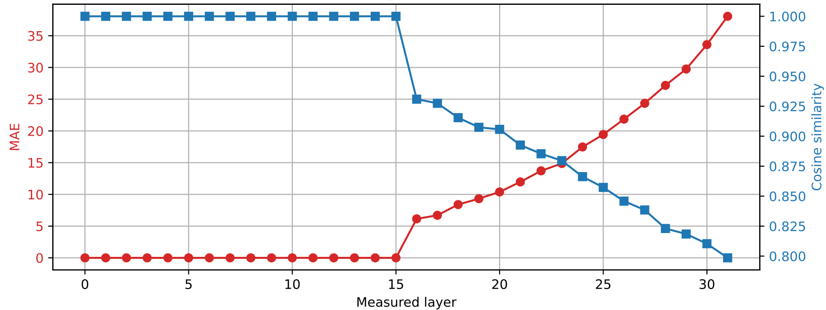
SmolLM2-360M | Prompt 0 Spared layer 15 | Hybrid vs quantized
