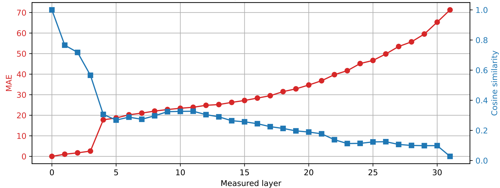
SmolLM2-360M | Prompt 0 Spared layer 17 | Hybrid vs unquantized
