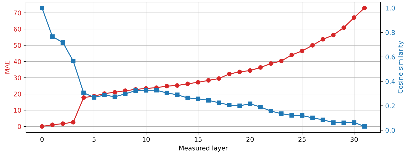
SmolLM2-360M | Prompt 0 Spared layer 19 | Hybrid vs unquantized
