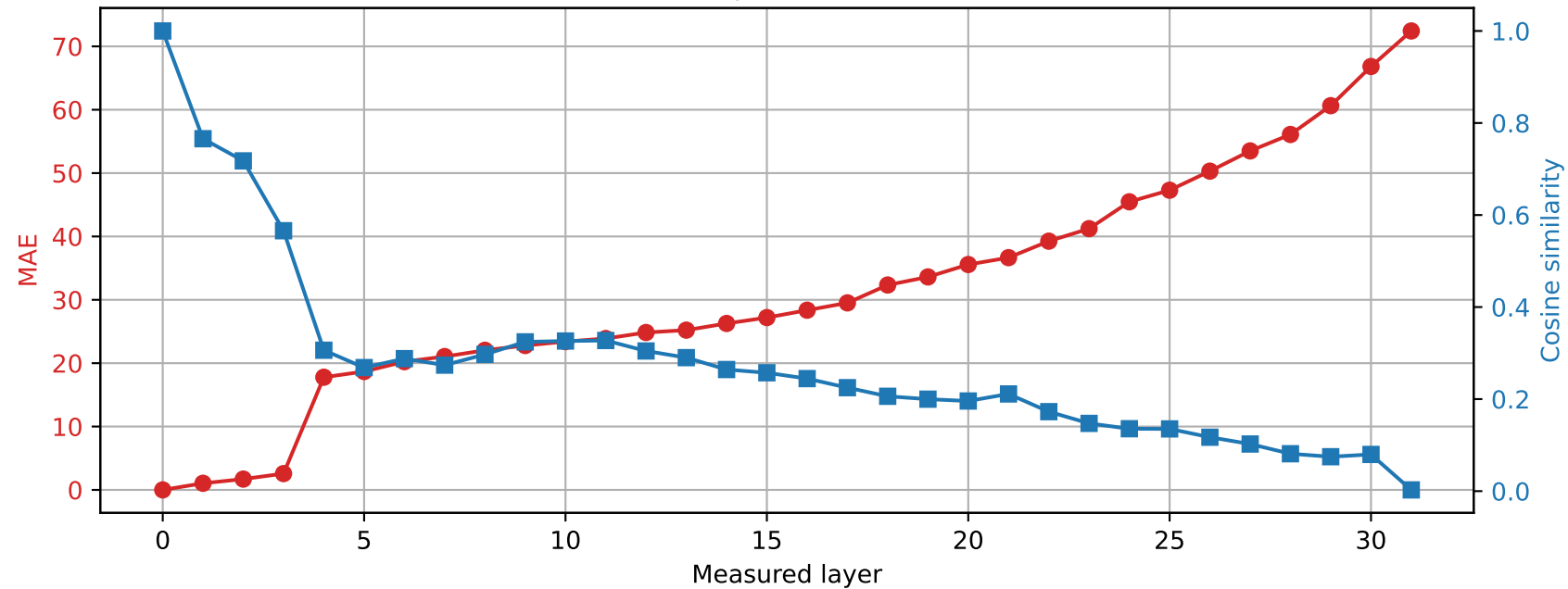
SmolLM2-360M | Prompt 0 Spared layer 20 | Hybrid vs unquantized
