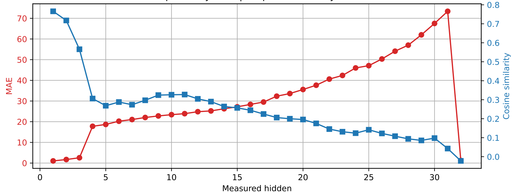
SmolLM2-360M | Prompt 0 Spared layer 24 | Unquantized vs hybrid
