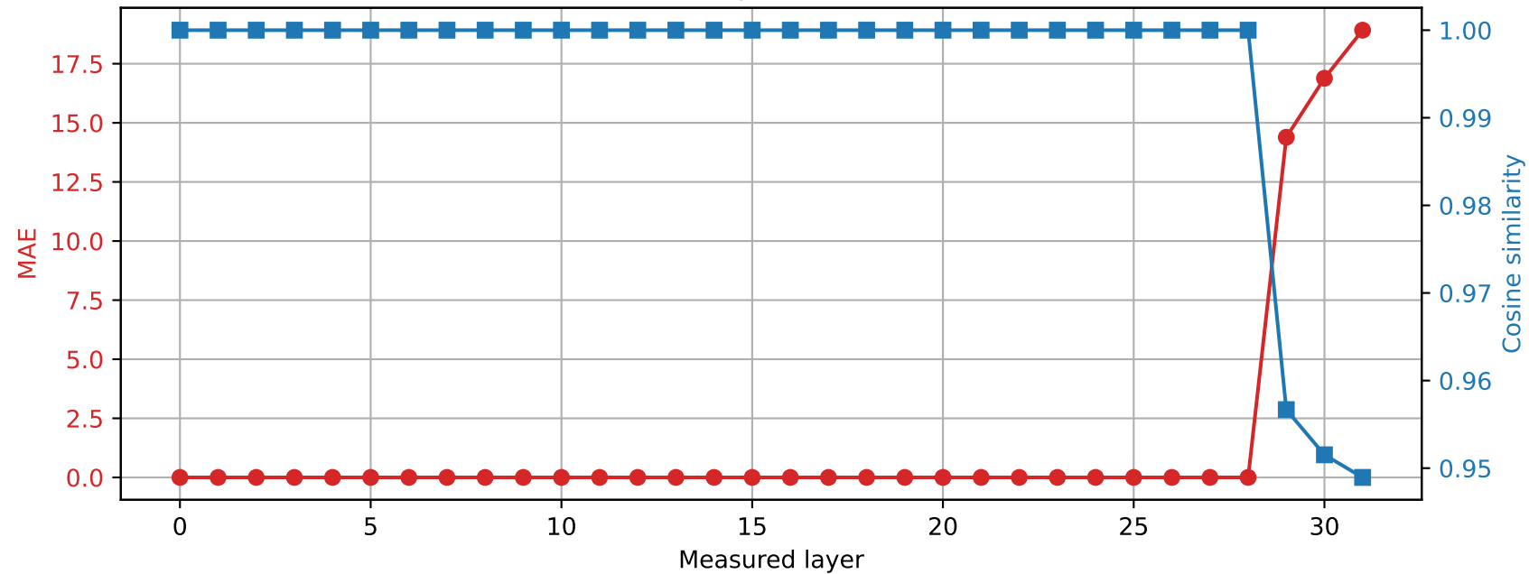
SmolLM2-360M | Prompt 0 Spared layer 28 | Hybrid vs quantized
