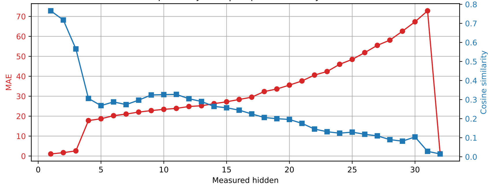
SmolLM2-360M | Prompt 0 Spared layer 29 | Unquantized vs hybrid
