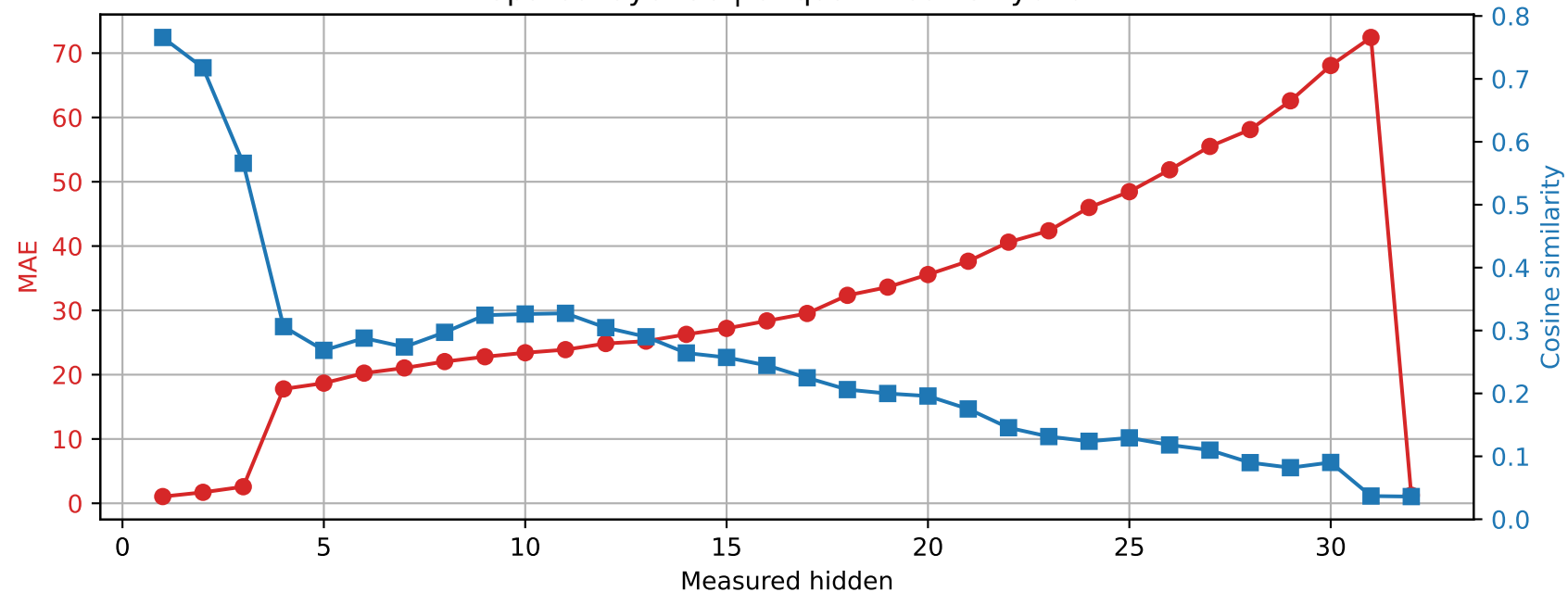
SmolLM2-360M | Prompt 0 Spared layer 30 | Unquantized vs hybrid
