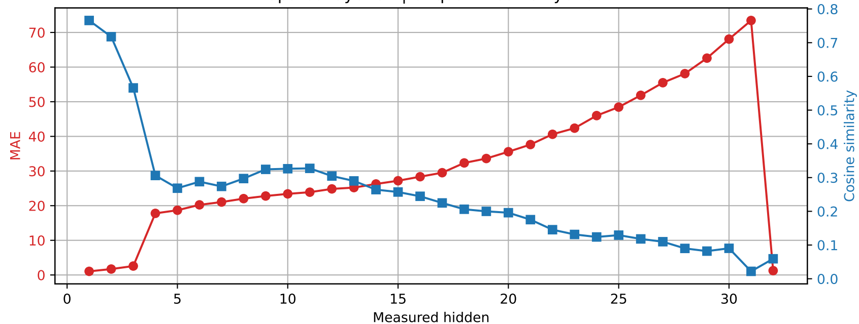
SmolLM2-360M | Prompt 0 Spared layer 31 | Unquantized vs hybrid
