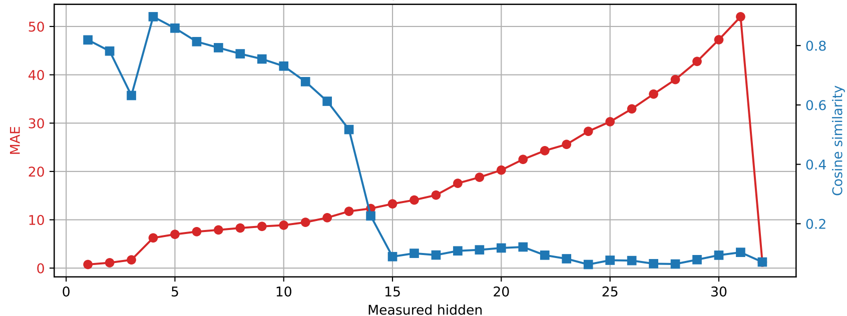
SmolLM2-360M | Prompt 1 Spared layer 5 | Unquantized vs hybrid
