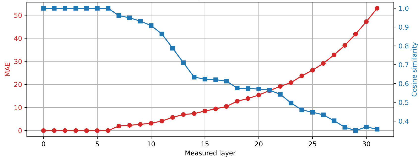
SmolLM2-360M | Prompt 1 Spared layer 6 | Hybrid vs quantized
