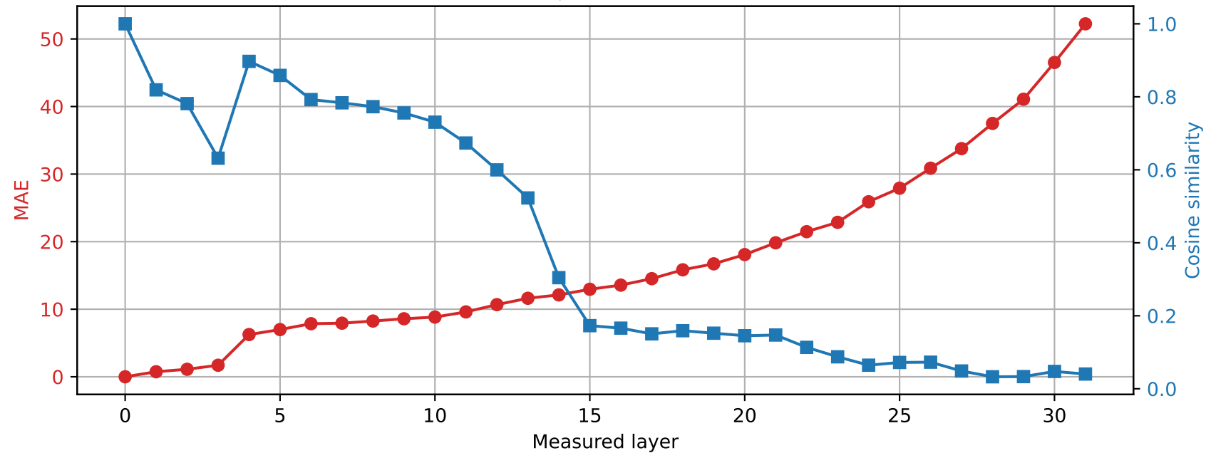
SmolLM2-360M | Prompt 1 Spared layer 6 | Hybrid vs unquantized
