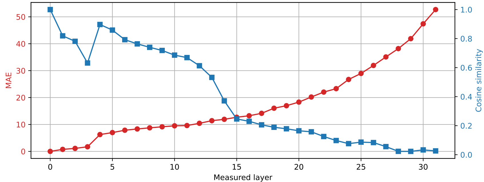
SmolLM2-360M | Prompt 1 Spared layer 10 | Hybrid vs unquantized
