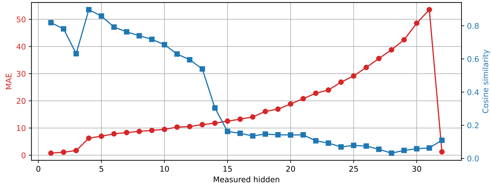
SmolLM2-360M | Prompt 1 Spared layer 11 | Unquantized vs hybrid
