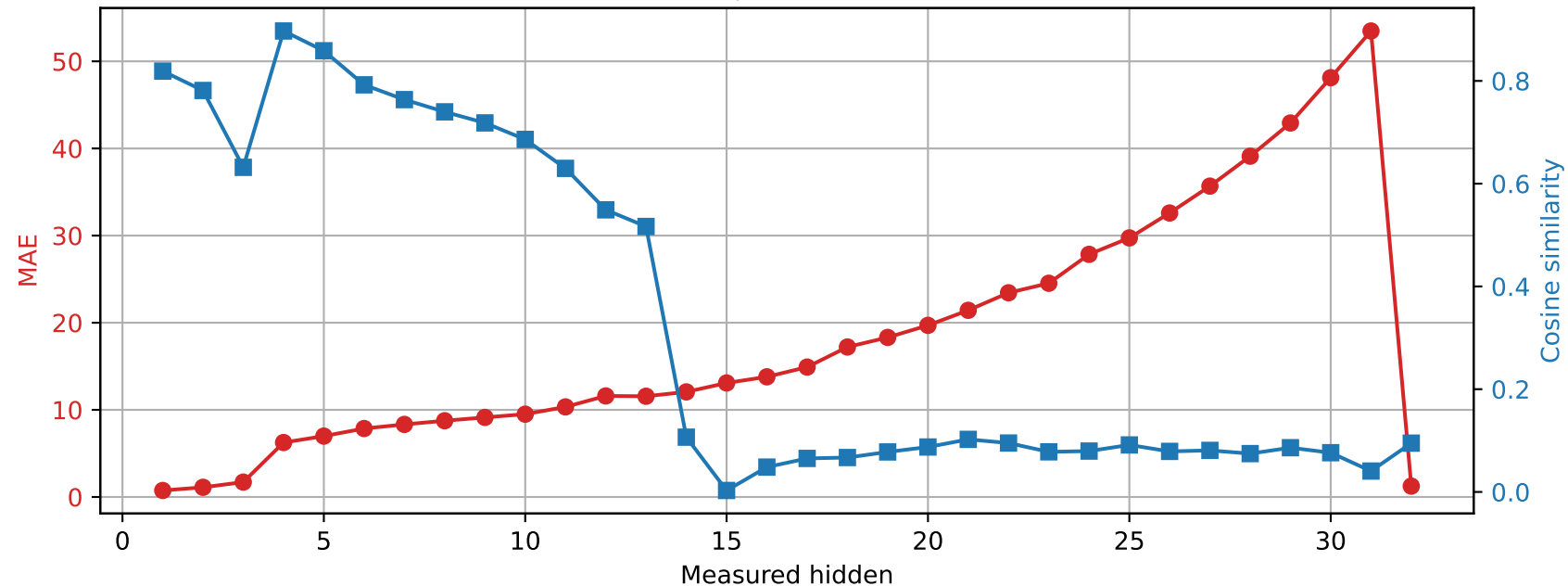
SmolLM2-360M | Prompt 1 Spared layer 12 | Unquantized vs hybrid
