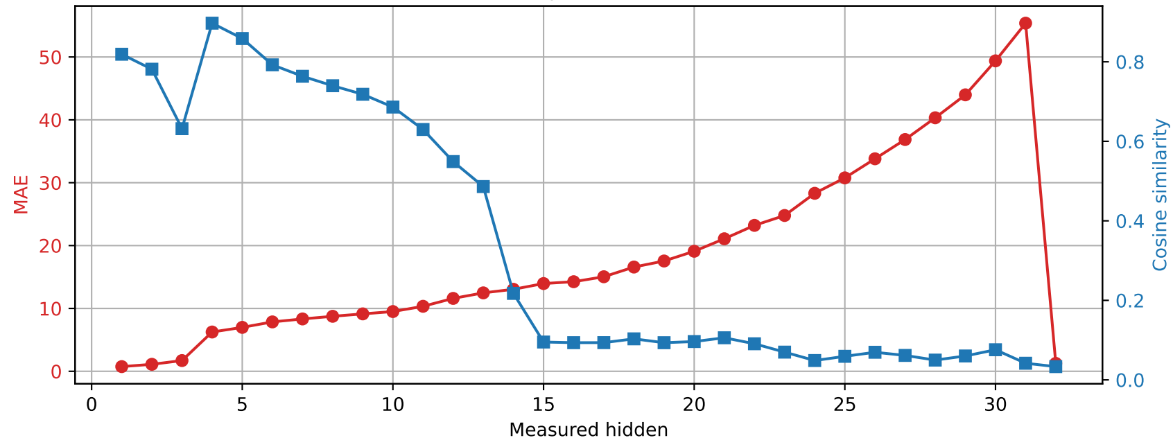
SmolLM2-360M | Prompt 1 Spared layer 15 | Unquantized vs hybrid
