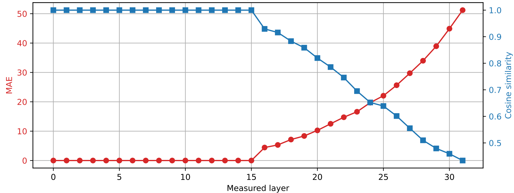
SmolLM2-360M | Prompt 1 Spared layer 15 | Hybrid vs quantized
