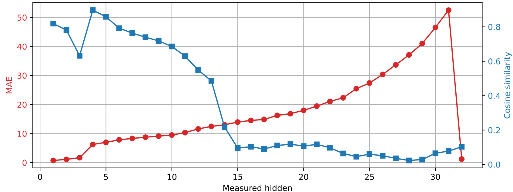
SmolLM2-360M | Prompt 1 Spared layer 16 | Unquantized vs hybrid
