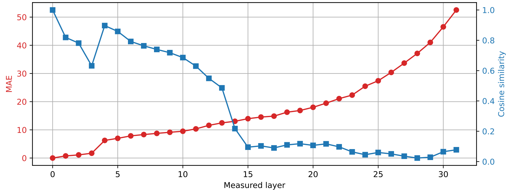
SmolLM2-360M | Prompt 1 Spared layer 16 | Hybrid vs unquantized
