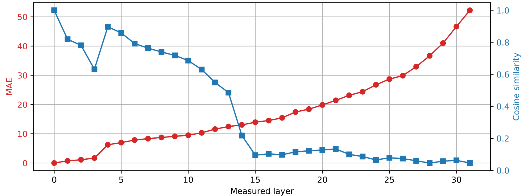
SmolLM2-360M | Prompt 1 Spared layer 25 | Hybrid vs unquantized
