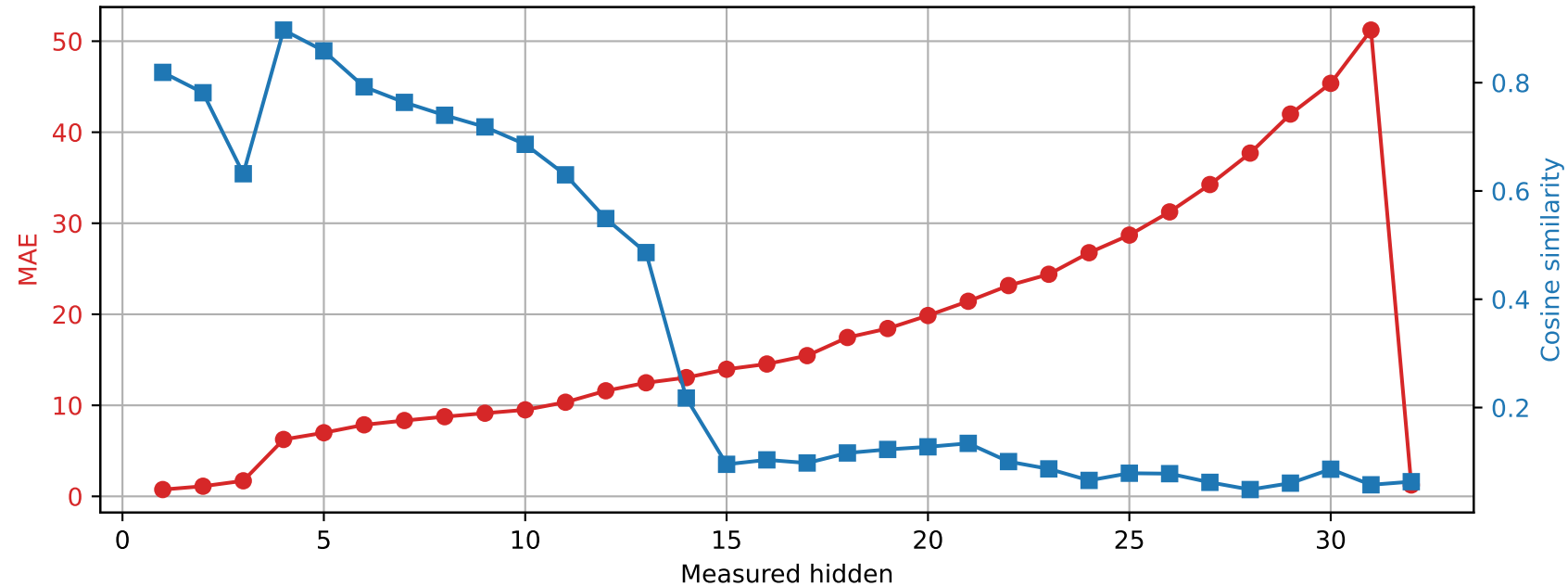
SmolLM2-360M | Prompt 1 Spared layer 29 | Unquantized vs hybrid
