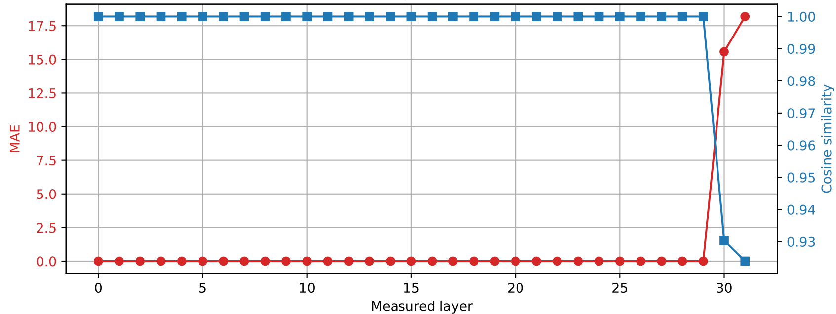
SmolLM2-360M | Prompt 1 Spared layer 29 | Hybrid vs quantized
