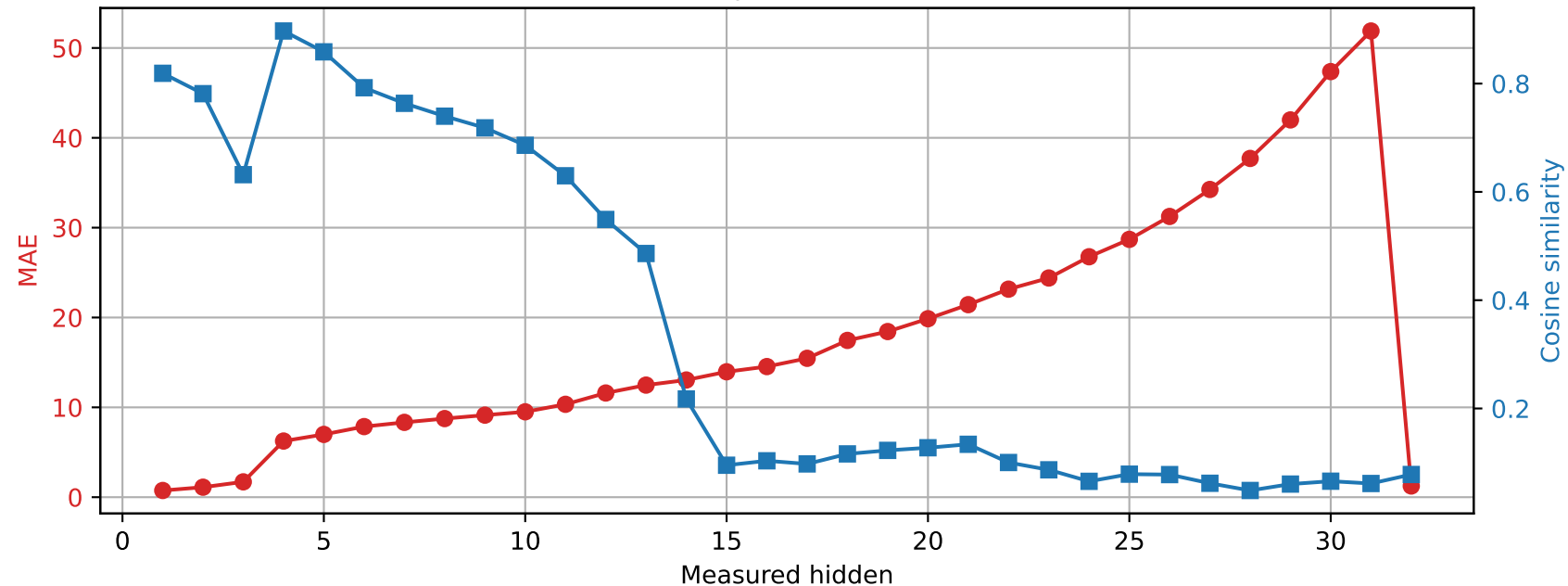
SmolLM2-360M | Prompt 1 Spared layer 30 | Unquantized vs hybrid
