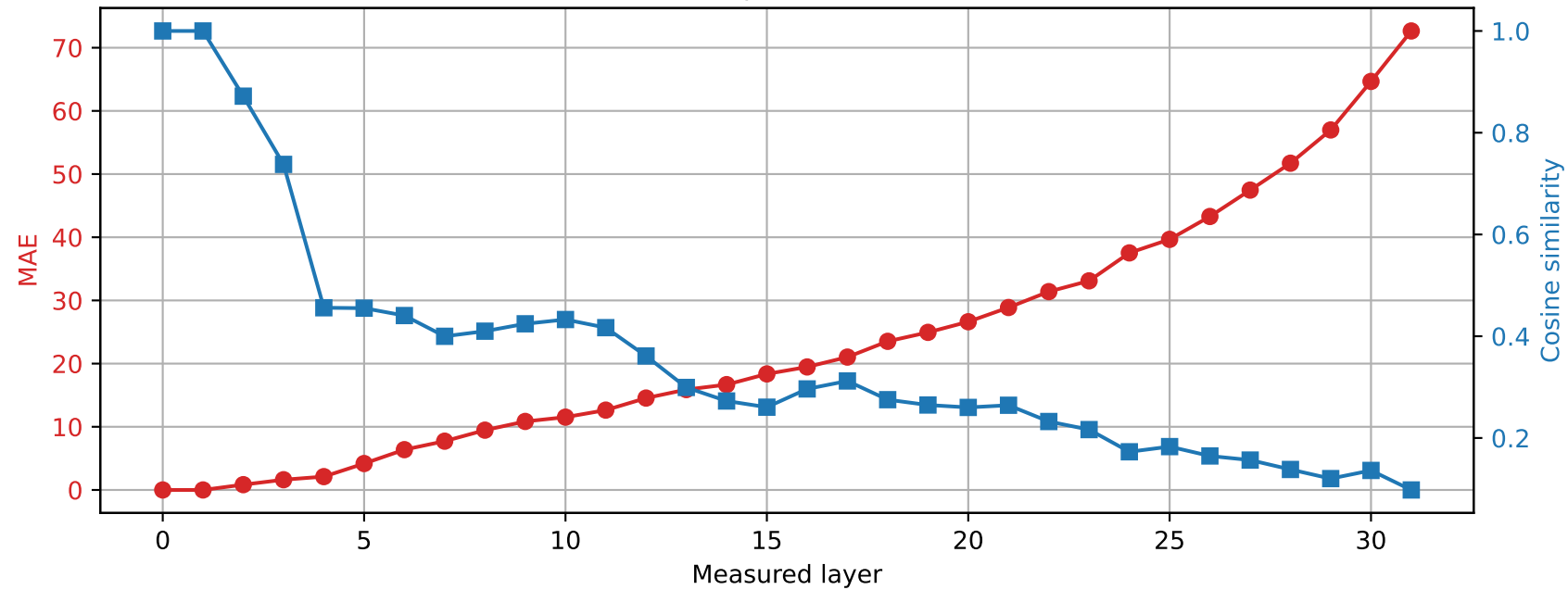
SmolLM2-360M | Prompt 2 Spared layer 1 | Hybrid vs quantized
