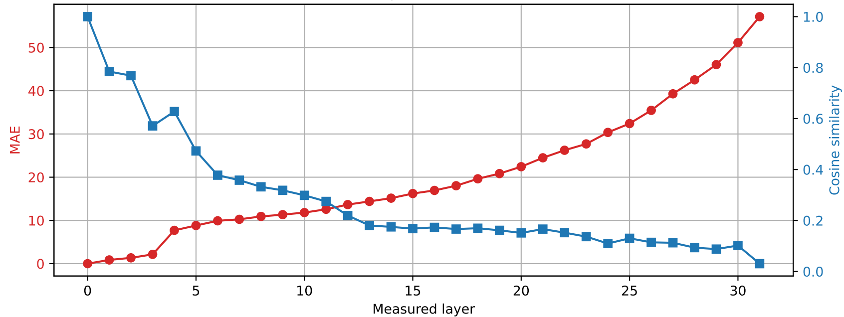
SmolLM2-360M | Prompt 2 Spared layer 6 | Hybrid vs unquantized
