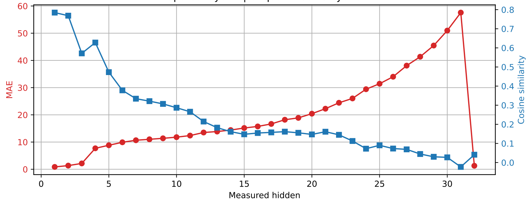
SmolLM2-360M | Prompt 2 Spared layer 7 | Unquantized vs hybrid
