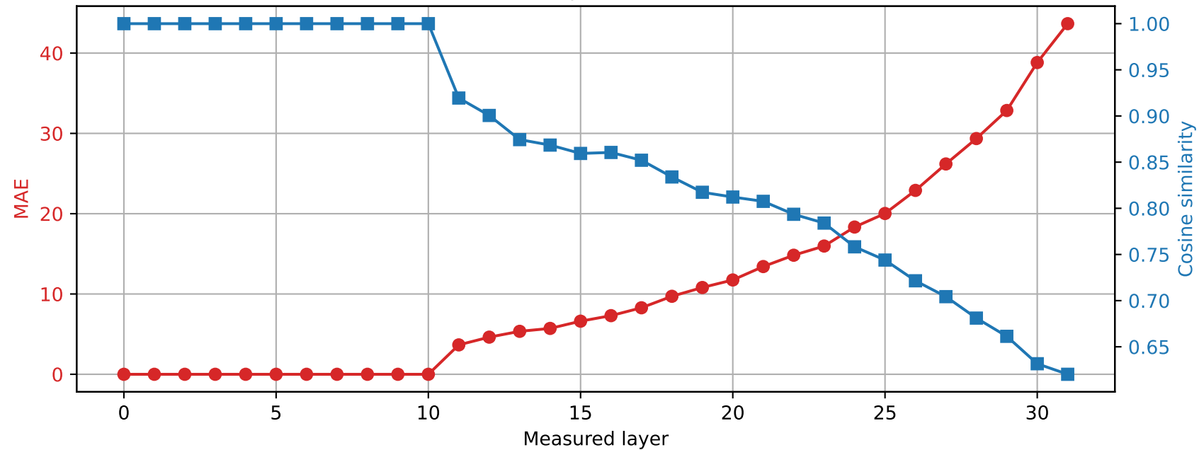
SmolLM2-360M | Prompt 2 Spared layer 10 | Hybrid vs quantized
