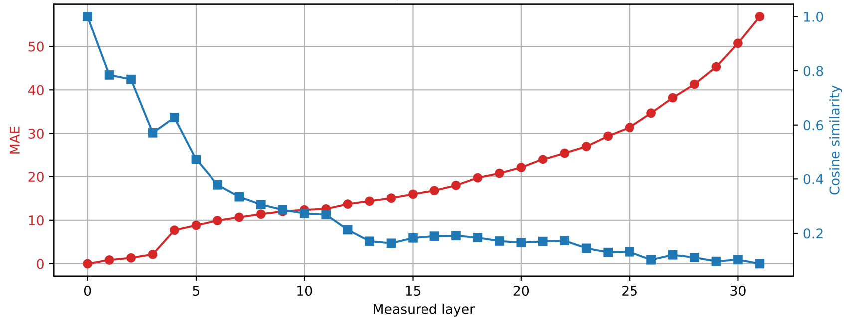
SmolLM2-360M | Prompt 2 Spared layer 10 | Hybrid vs unquantized
