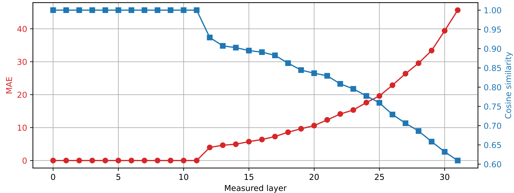
SmolLM2-360M | Prompt 2 Spared layer 11 | Hybrid vs quantized
