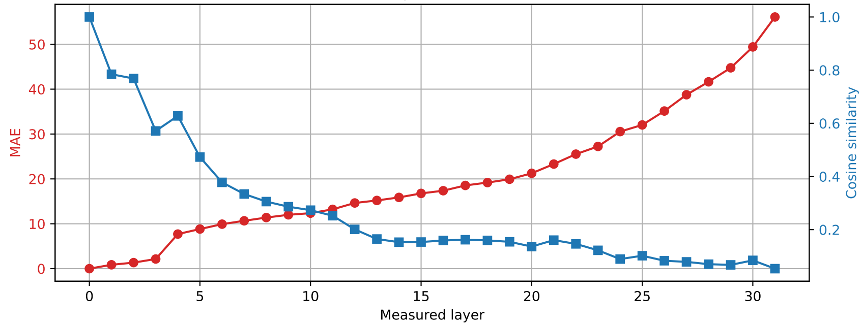
SmolLM2-360M | Prompt 2 Spared layer 17 | Hybrid vs unquantized
