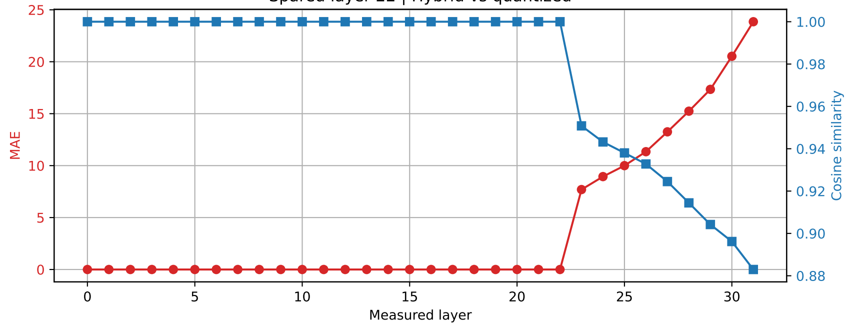
SmolLM2-360M | Prompt 2 Spared layer 22 | Hybrid vs quantized
