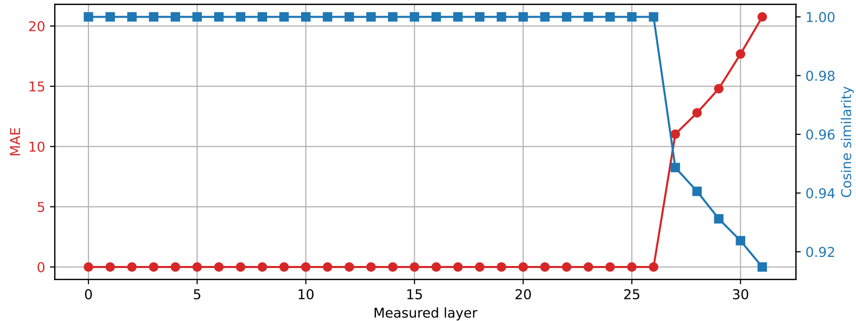
SmolLM2-360M | Prompt 2 Spared layer 26 | Hybrid vs quantized
