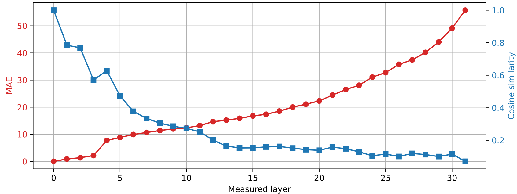
SmolLM2-360M | Prompt 2 Spared layer 26 | Hybrid vs unquantized
