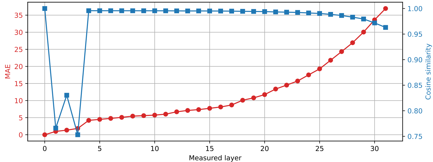
SmolLM2-360M | Prompt 3 Spared layer 1 | Hybrid vs unquantized
