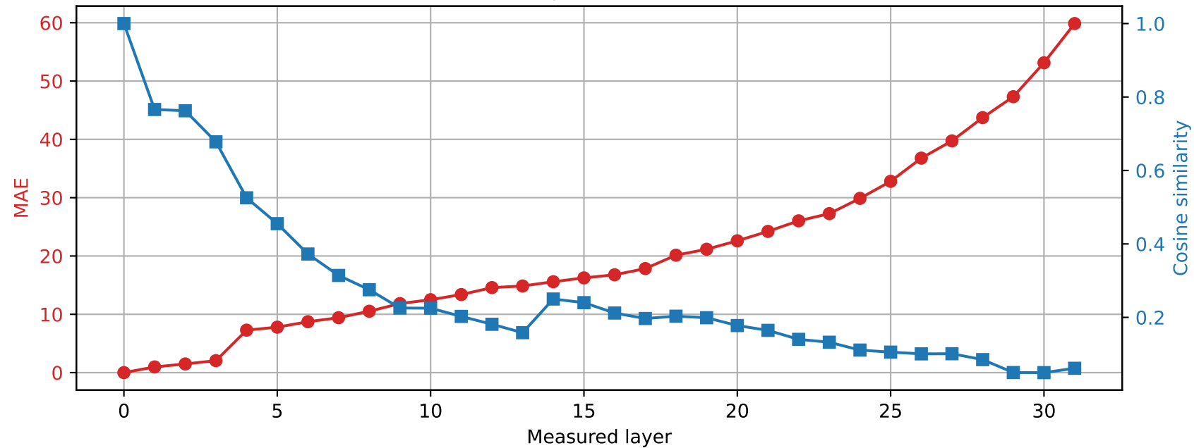
SmolLM2-360M | Prompt 3 Spared layer 3 | Hybrid vs unquantized
