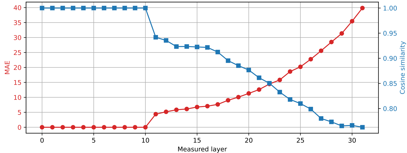
SmolLM2-360M | Prompt 3 Spared layer 10 | Hybrid vs quantized
