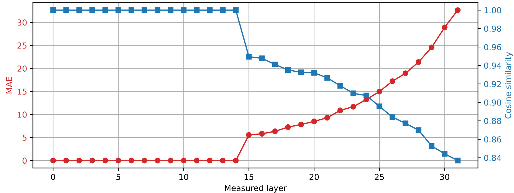
SmolLM2-360M | Prompt 3 Spared layer 14 | Hybrid vs quantized
