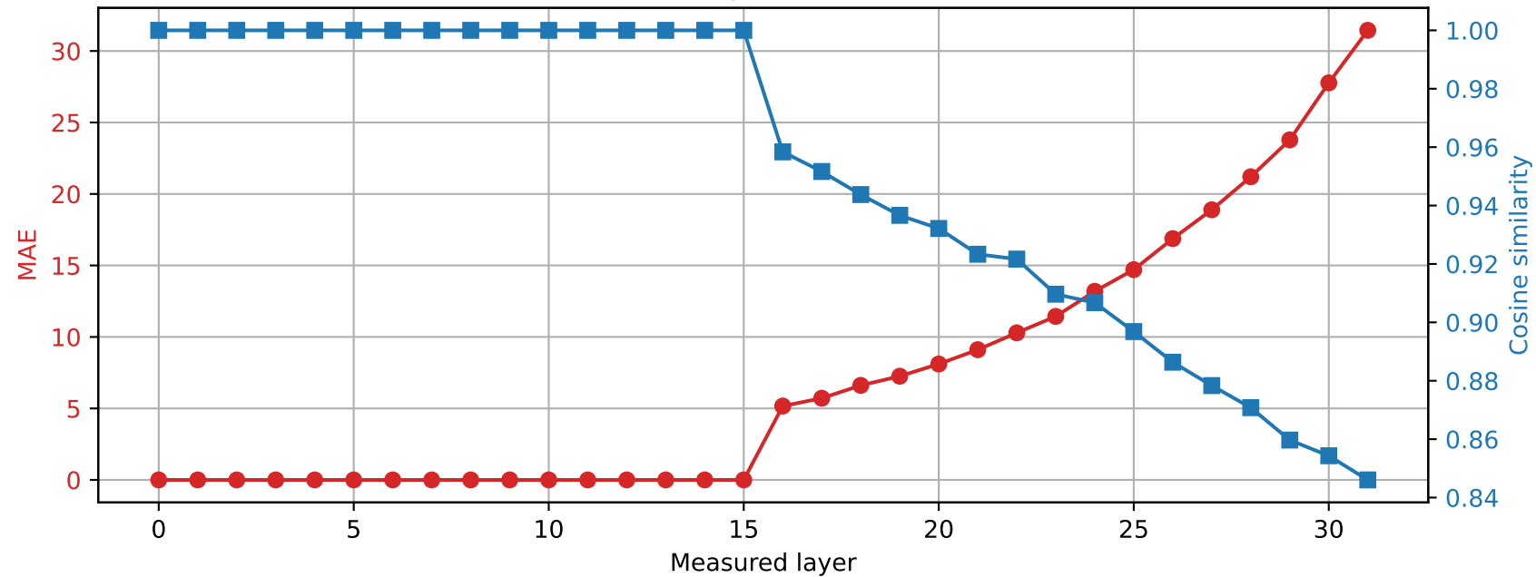
SmolLM2-360M | Prompt 3 Spared layer 15 | Hybrid vs quantized
