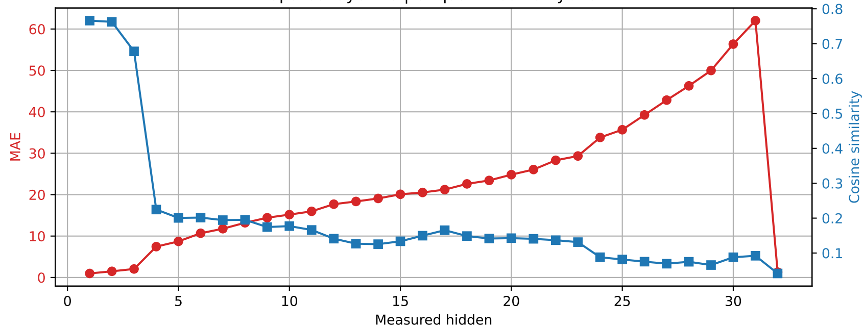
SmolLM2-360M | Prompt 3 Spared layer 16 | Unquantized vs hybrid
