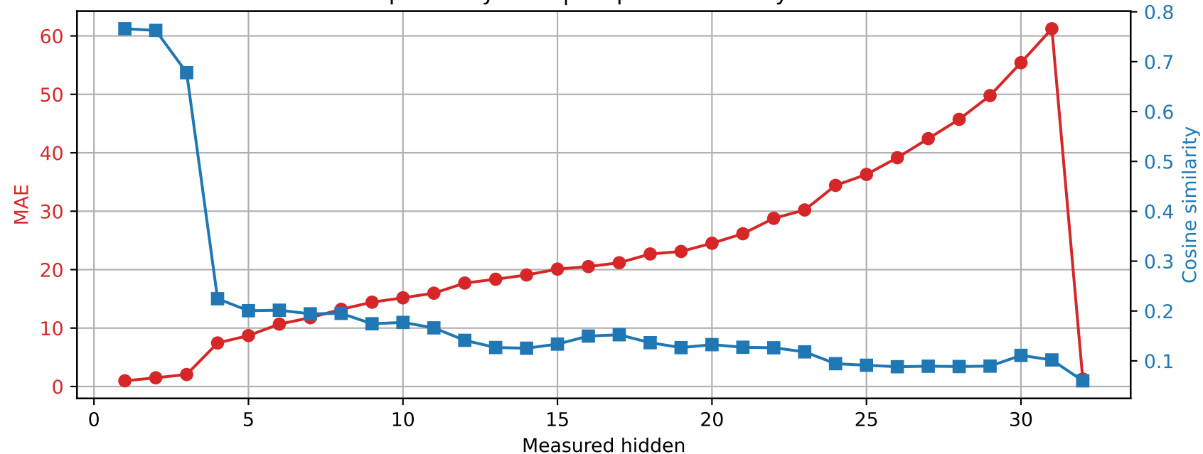
SmolLM2-360M | Prompt 3 Spared layer 18 | Unquantized vs hybrid
