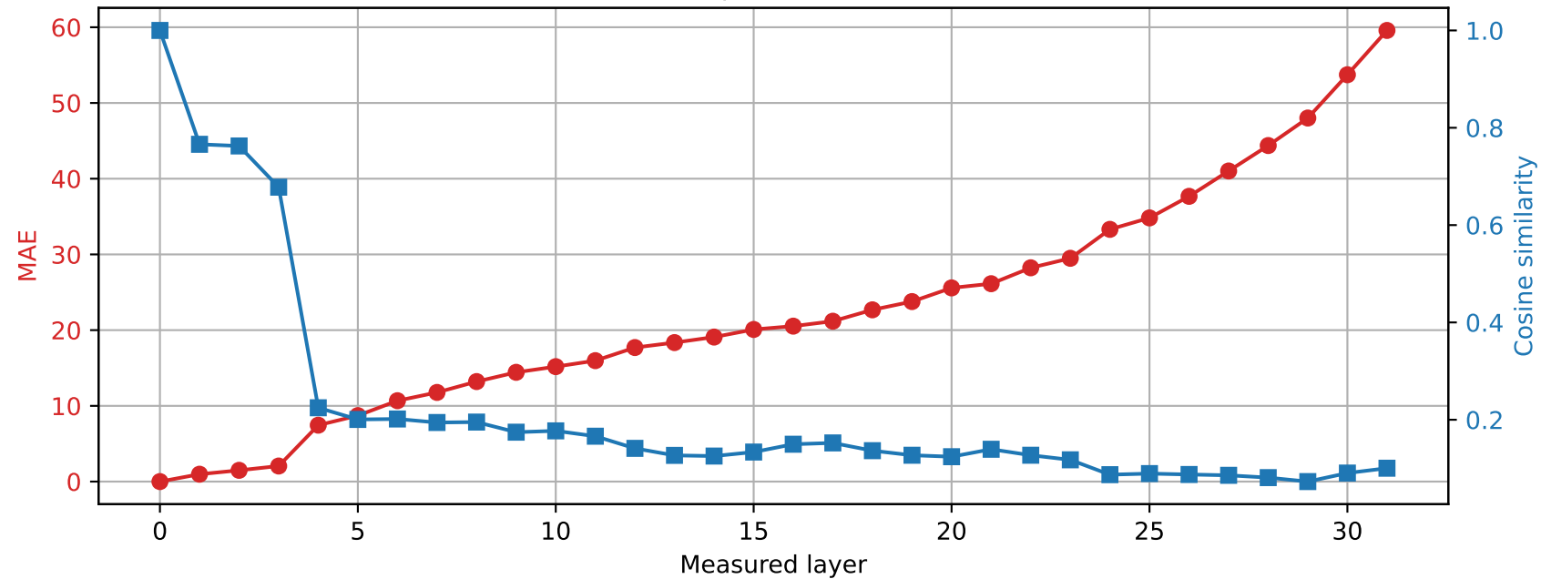
SmolLM2-360M | Prompt 3 Spared layer 20 | Hybrid vs unquantized
