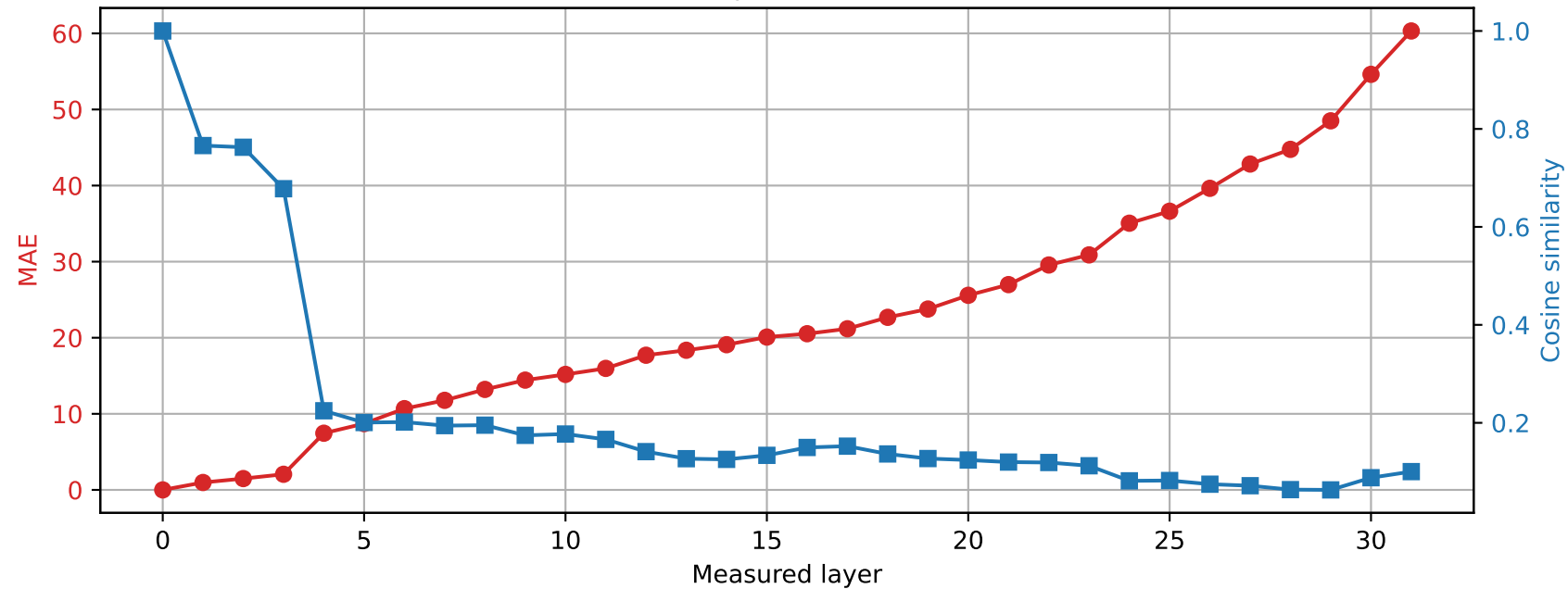
SmolLM2-360M | Prompt 3 Spared layer 27 | Hybrid vs unquantized
